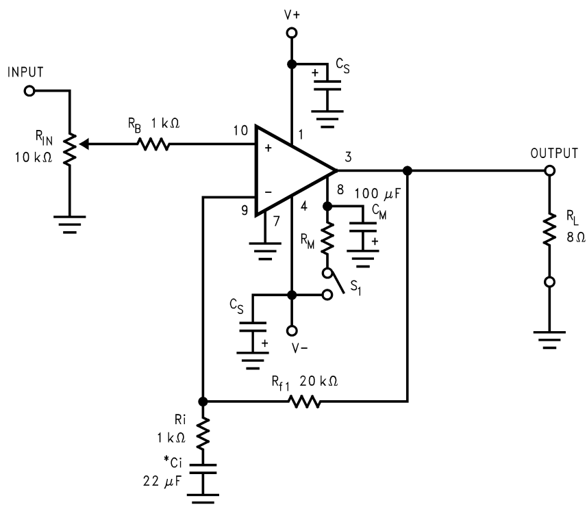
Figure 1. Typical Audio Amplifier Application Circuit
